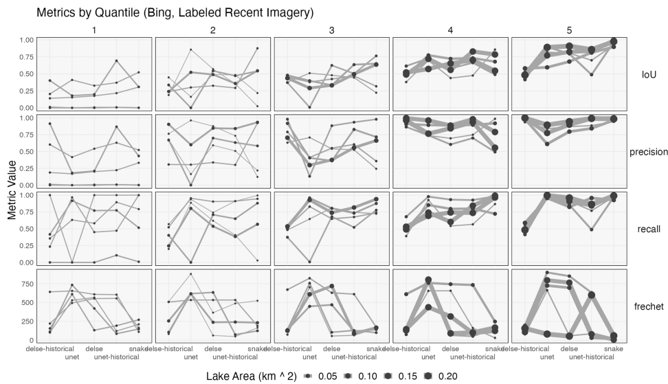
Fig. 2. Analog of Fig. 2 generated for newly labeled high-resolution imagery. Models are again sorted from those with lowest to highest average IoU, though note that the order has changed.
