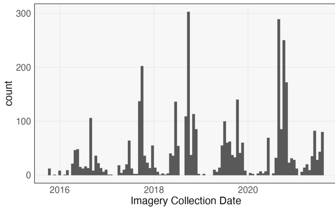
Fig. 10. Sentinel 2 imagery collection date. More imagery is available in recent years. Since labels were created in a 2015 study, only images from 2015 to 2016 were used for training and evaluation.
