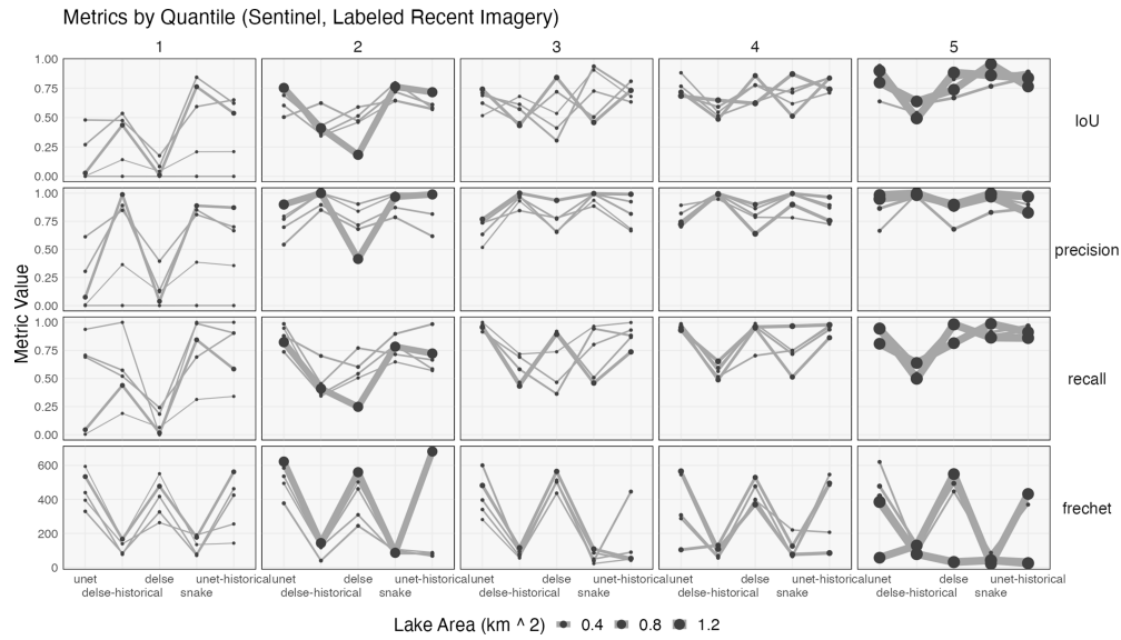
Fig. 1. Comparison of lakewise performance across models when evaluating with newly labeled Sentinel 2 imagery. Each column corresponds to one quantile of lake performance (lowest to highest performance from left to right), and each row is a performance metric. The five lines in each panel correspond to five randomly selected lakes within that quantile. Models are sorted from those with lowest average IoU to those with the highest average IoU.
