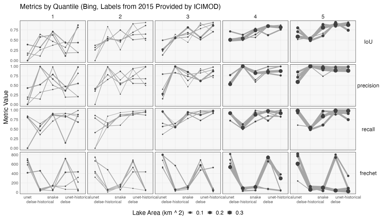
Fig. 12. Analog of Fig. 2 for the error with respect to 2015 ICIMOD labels for lakes within the Bing test set. These 2015 labels are more plentiful, but not as accurate on the recently collected Bing imagery.
