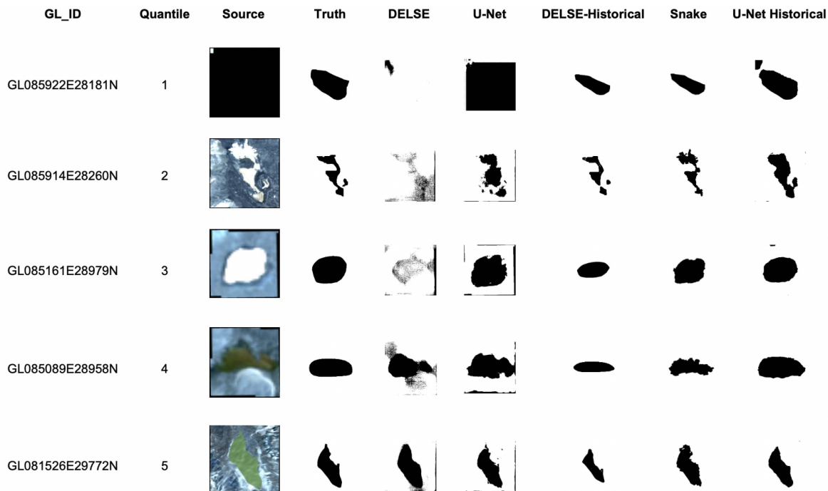
Fig. 13. Example lake predictions taken from the quantiles shown in Appendix Fig. 11. The ground truth shown here are those from the 2015 ICIMOD survey. The lake from the highest error quantile is masked by a no-data region of a Sentinel 2 tile.
