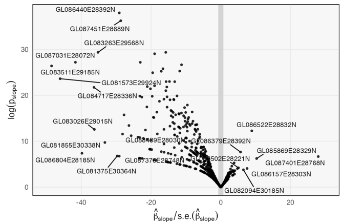
Fig. 7. Volcano plot of estimated glacial lake area changes. Lakes at the bottom of the “V” do not have detectable trends in glacial lake area. Those on the upper right (left) have significant increasing (decreasing) areas. Two example glacial lakes labeled here are shown in Fig. 8.
